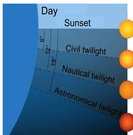
Fig. 2. Three types of twilight
