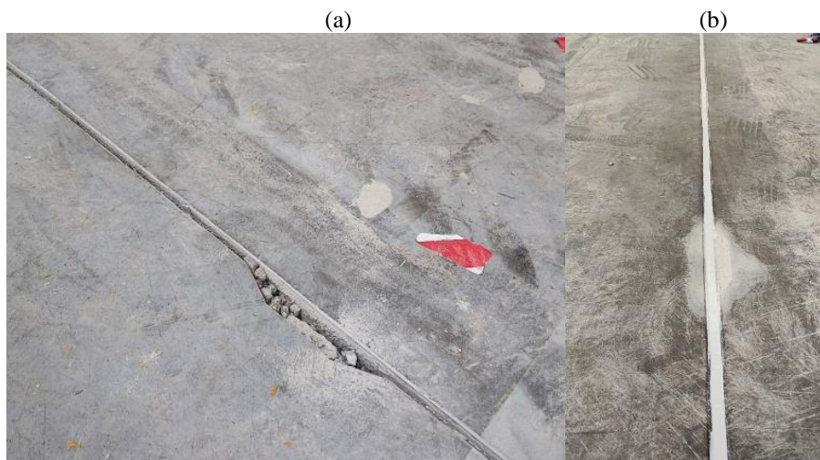
Fig. 19. Concrete industrial floor (Example 4) during repair: a) visible loss of expansion joint edge, b) spot repair of expansion joint edge with restoration of infill [38]
