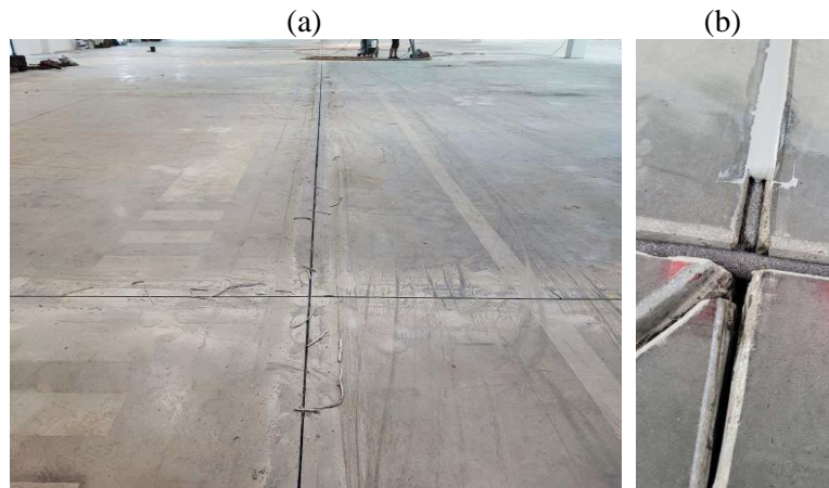
Fig. 18. Concrete industrial floor (Example 4) during repair: a) removal of degraded shrinkage joint fill, b) placement of new shrinkage joint fill [38]
